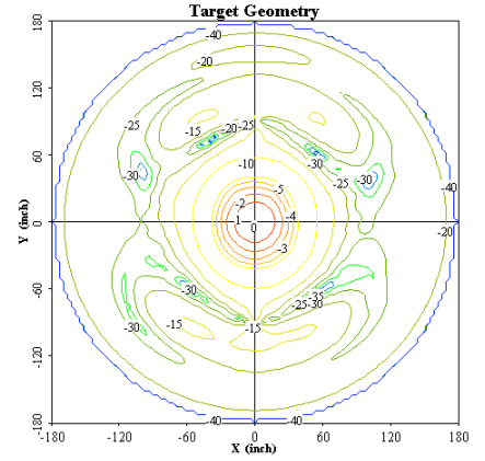
Color Contour
