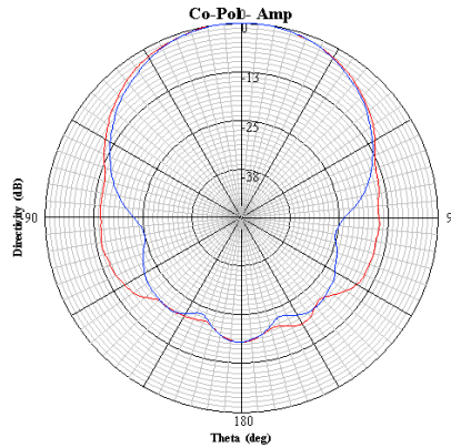
Polar 3D
