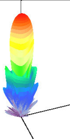
Polar 3D
